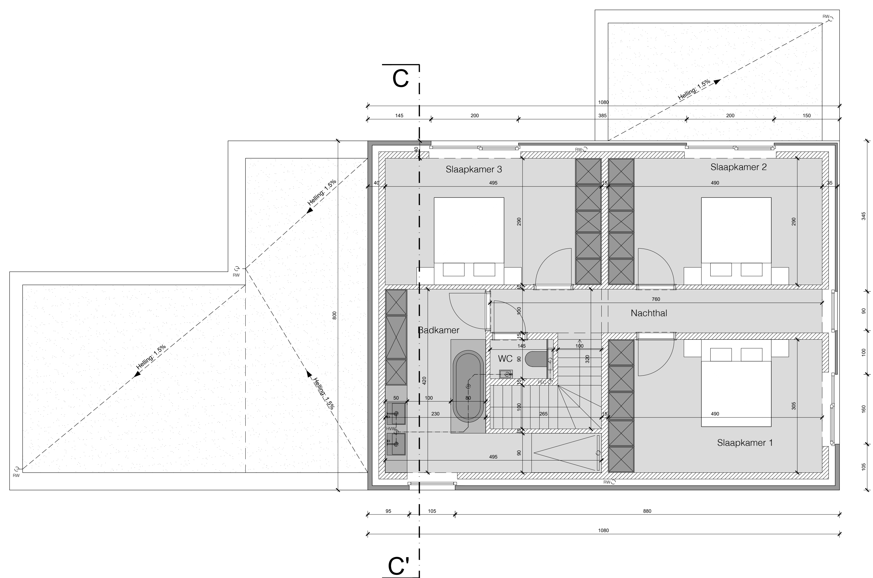
plan VERDIEPING +1 1/50
